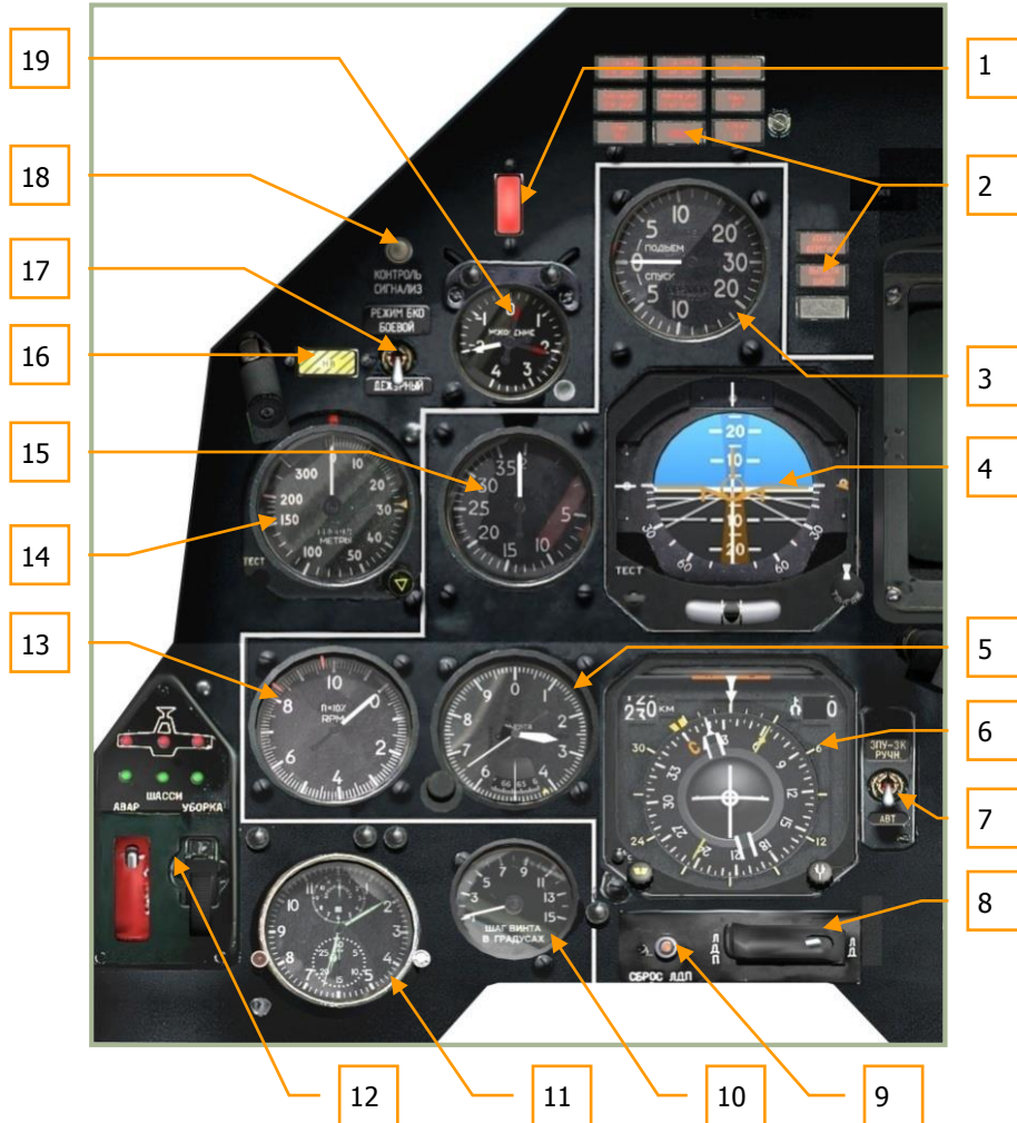
6-9: Linkes Frontpanel
