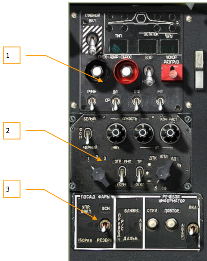
6-38: Mittleres Panel
